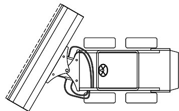
Hydraulic tilting
